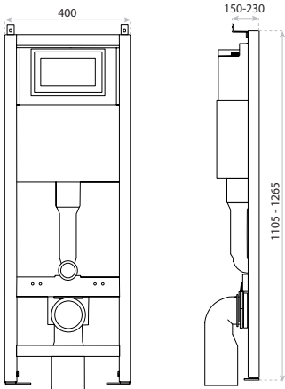
FRAME FOR CONCEALED INSTALLATION OF A TOILET LAV 101 DIMENSIONS (MM) 1105-1265 x 400 x 150-230 EAN 5908211494838
